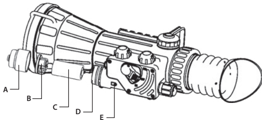
FIGURE 3-1. VULCAN BATTERY INSTALLATION
